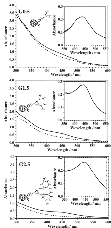
Figure 1. UV–vis absorption spectra of C_{60}(Gn-COOK) (broken line) and Ag-C_{60}(Gn-COOK) nanoparticles (solid line) in water. Insets: differential spectra and chemical structures of fullerodendrons.
